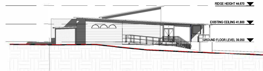
3 SOUTHERN ELEVATION - NOTIFICATION PLAN
